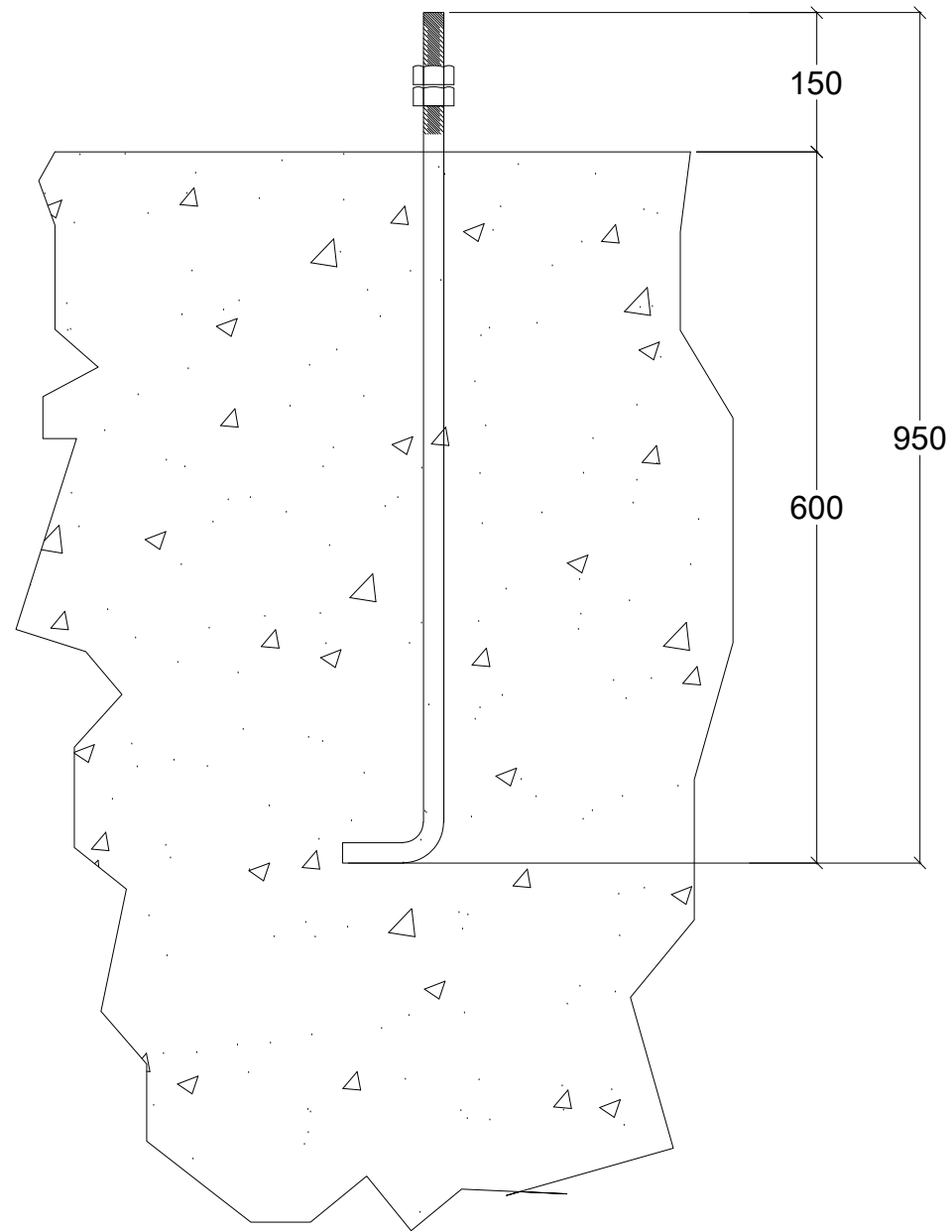
DETAIL OF Foundation Bolts M-24X950mm HD BOLTS = 144 sets
